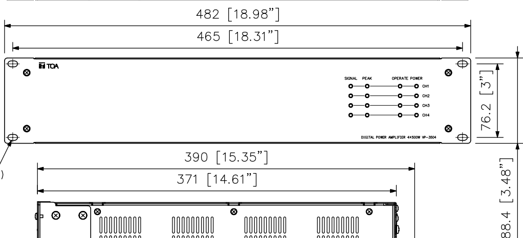
Front View
